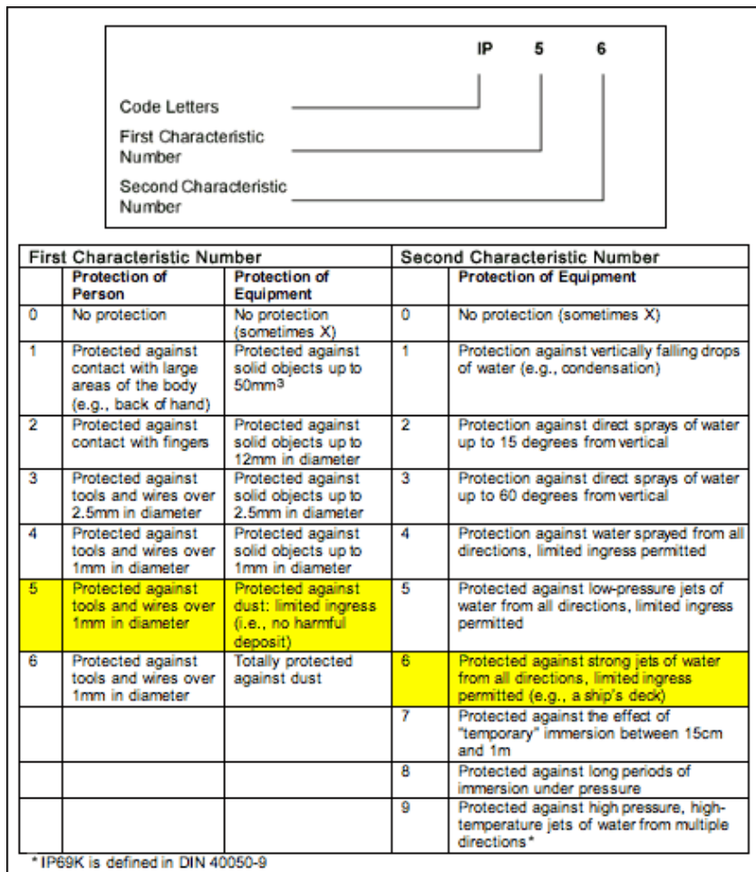
Figure 1. IP rating format.
